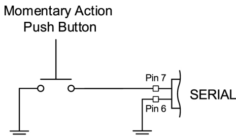
Figure: Contact Closure Style Trigger Button Circuit Diagram (SYNC)
